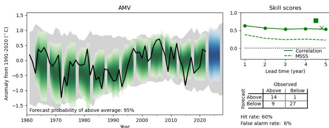
Figure 5: Multi-annual predictions of Atlantic Multidecadal Variability (AMV) relative to its 1991-2020 average, defined as the anomaly difference between two regions: 45^{\circ}\text{N} - 60^{\circ}\text{N} , 60^{\circ}\text{W} - 0^{\circ}\text{E} minus 45^{\circ}\text{S} - 0^{\circ}\text{S} , 30^{\circ}\text{W} - 10^{\circ}\text{E} as in Roberts et al (2013). Annual mean observations (see Figure 3) in black, forecast in blue, hindcasts in green and uninitalised simulations in grey. The shading indicates the 90% confidence range. The calibrated probability for the most likely category (above or below climatology) of the five-year-mean forecast is given at the bottom of the main panel. Hindcast skill scores are shown in the
