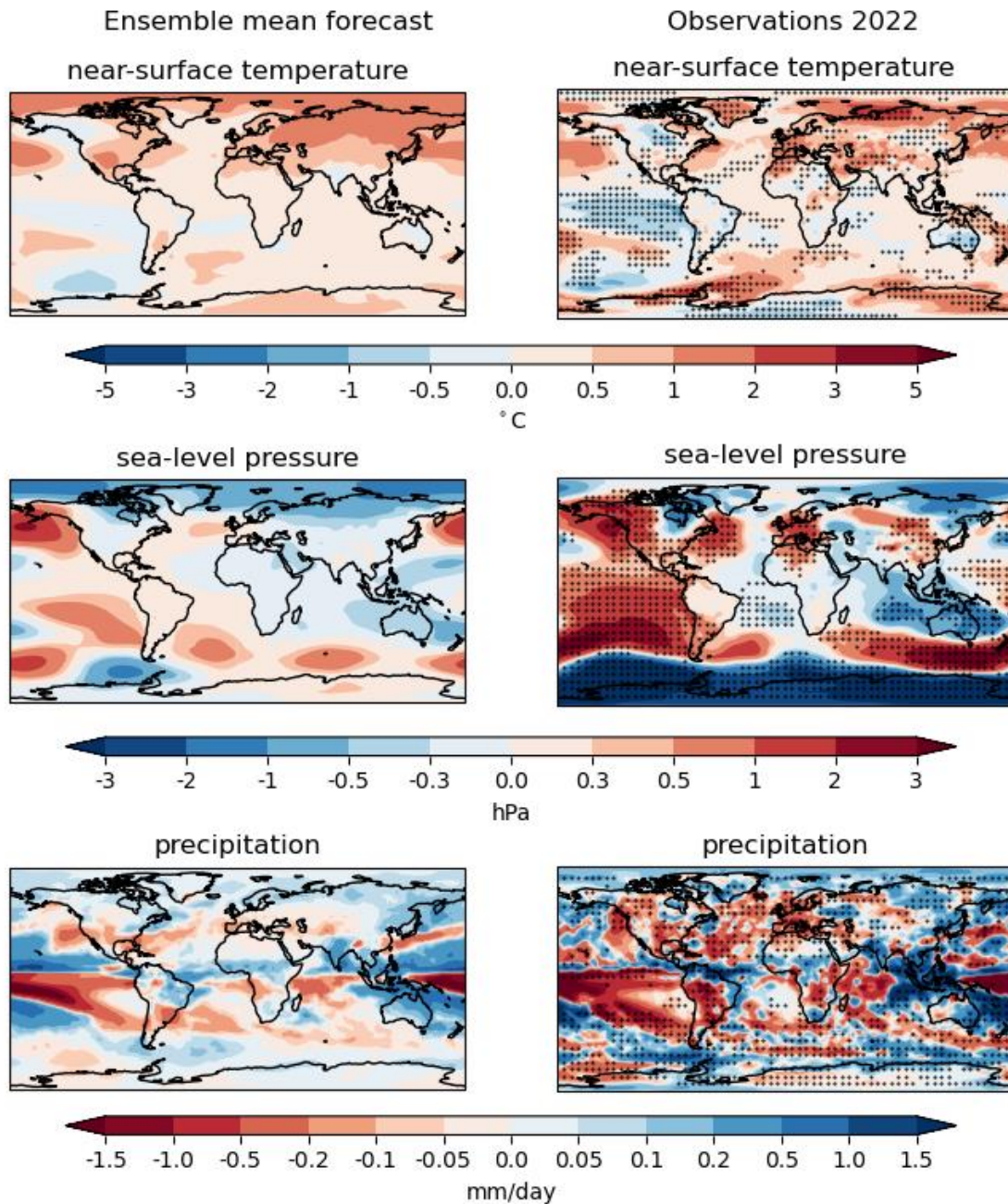
Figure 15: Evaluation of the one-year forecast for 2022 relative to 1981-2010. Ensemble mean forecast (left) and observed (right) anomalies. Top: temperature (°C); middle: sea level pressure (hPa); bottom: precipitation (mm/day). Stippling shows where the observations fall outside of the 90% range of the forecast ensemble.
