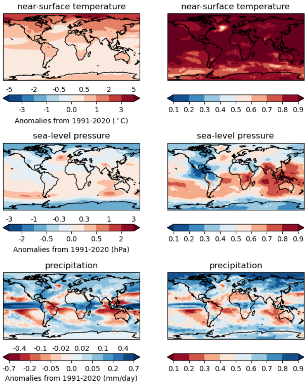
Figure 11: Predictions for 2023/2024-2027/2028 November to March anomalies relative to 1991-2020. Ensemble mean (left column) for temperature (top, °C), sea level pressure (middle, hPa), precipitation (bottom, mm/day) and probability of above average (right column). As this is an uncalibrated two-category forecast, the probability for below average is one minus the probability shown in the right column.
