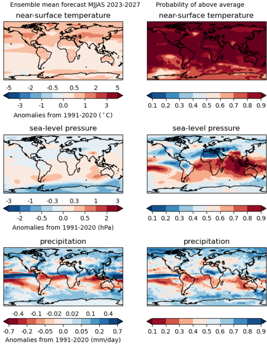
Figure 9: Predictions for 2023-2027 May to September anomalies relative to 1991-2020. Ensemble mean (left column) for temperature (top, ^{\circ}\text{C} ), sea level pressure (middle, hPa), precipitation (bottom, mm/day) and probability of above average (right column). As this is an uncalibrated two-category forecast, the probability for below average is one minus the probability shown in the right column.
