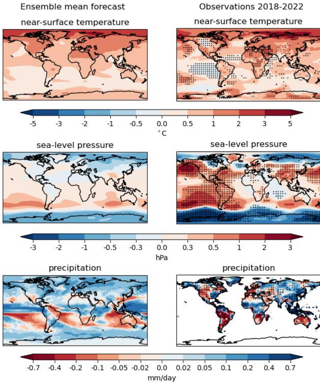
Figure 16: Evaluation of the five-year forecast for 2018-2022 relative to 1971-2000. Ensemble mean forecast (left) and observed (right) anomalies. Top: temperature (°C); middle: sea level pressure (hPa); bottom: precipitation (mm/day). Stippling shows where the observations fall outside of the 90% range of the forecast ensemble.
